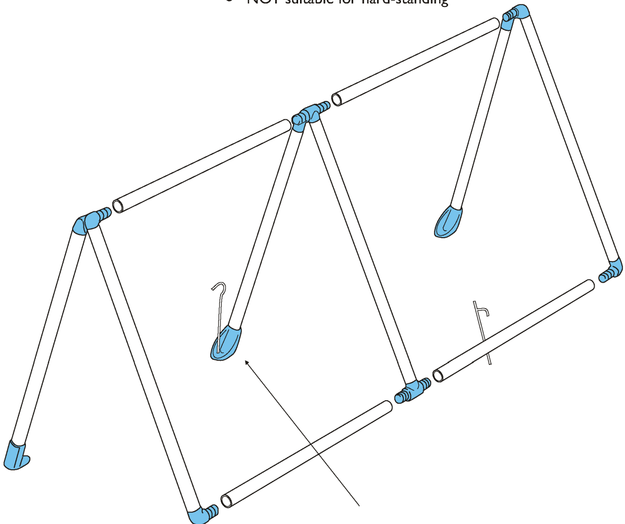
ROUND PLASTIC FEET FOR THE PEG TO PASS THROUGH
