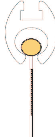
Fastrack keder can be sewn or welded to the perimeter
