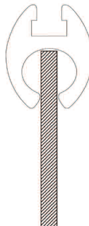
Support upto 5mm rigid panels
